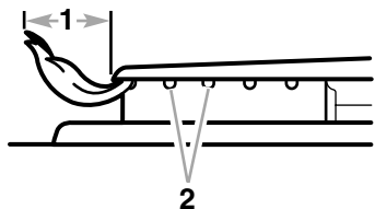
1. 1-1½ in. (25-38 mm) 2. Burner Ports
